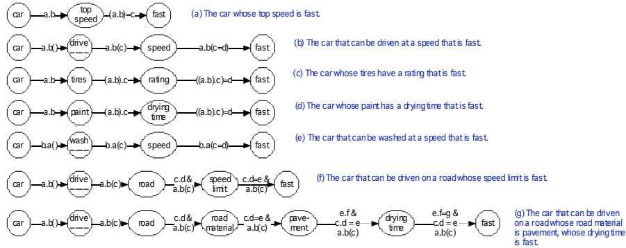
Figure 2. An underlying semantic model of English is used to generate interpretations of “fast car.” From [8].
